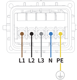
GRID terminal
