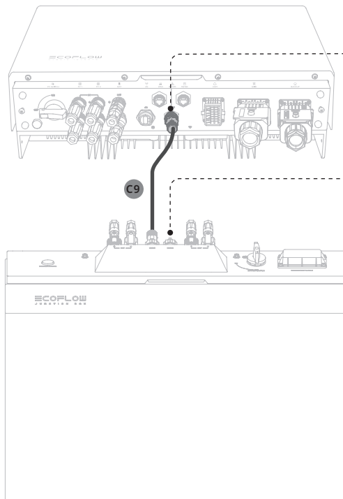
Battery communication port (BAT)
