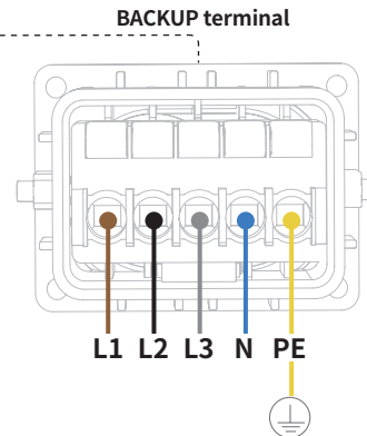
BACKUP terminal
